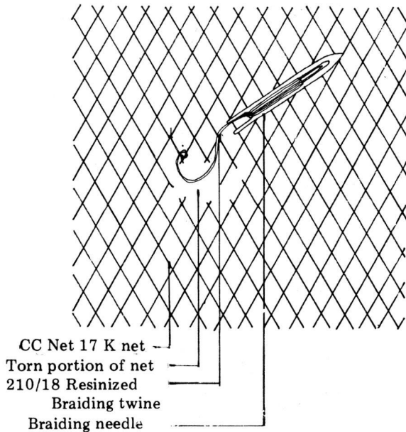
Fig. 16. Another technique in repairing net
