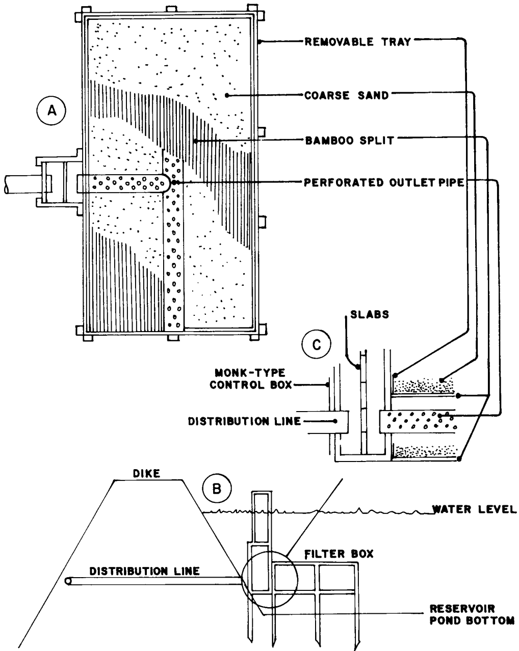
Fig. 2. Diagram showing filtration box in reservoir pond. A - Top view showing layers of coarse sand, and bamboo splits, B - side view of filter box in reservoir pond, C - Inset showing the details inside filter box and drain control box .
