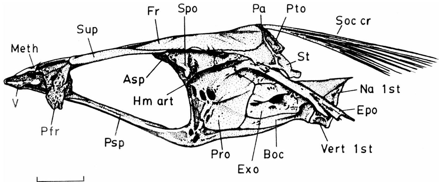
Fig. 2. Lateral view of the skull of milkfish, Chanos chanos Forsskal. (Scale represents 1 cm.)
