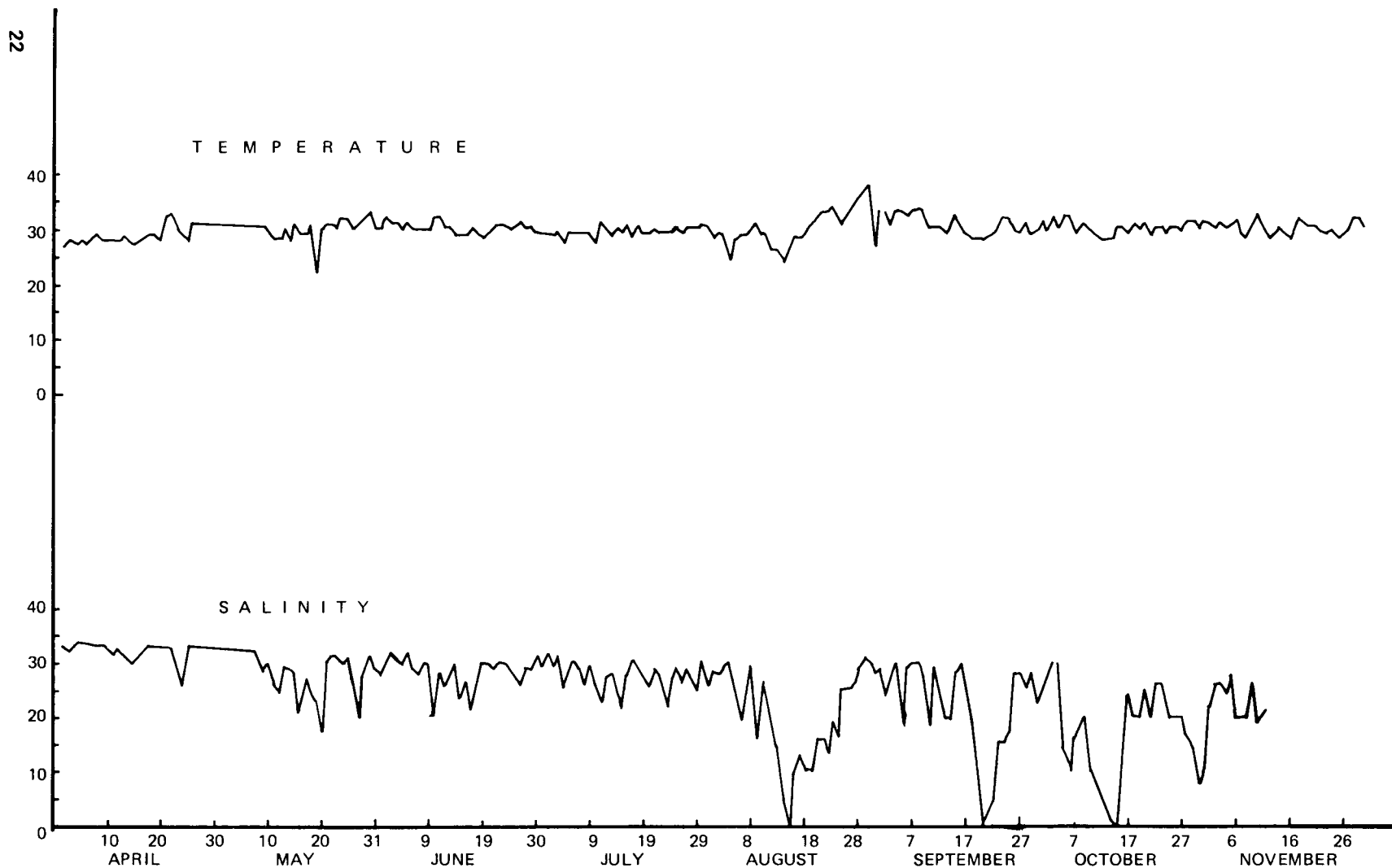
Fig. 3. Temperature and salinity conditions at Himamaylan River, April--November, 1981.
