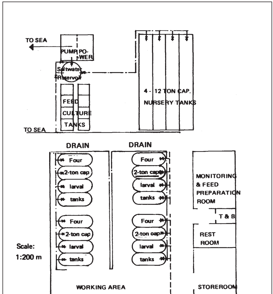
FIG. 1. Proposed layout for a small scale P. monodon hatchery.
