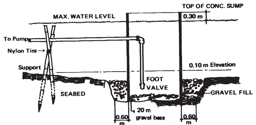
FIG. 2 Proposed detail of saltwater sump pit.
