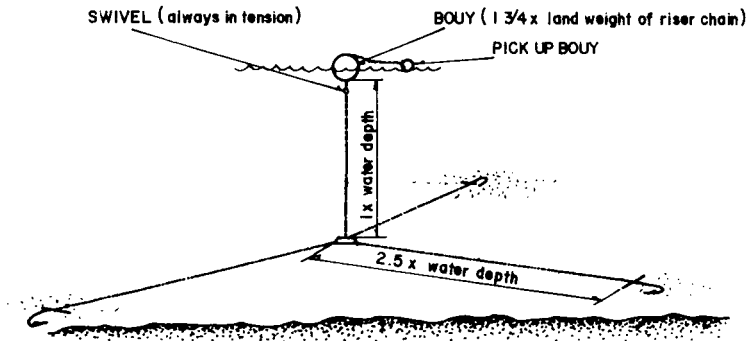
Single-point mooring
